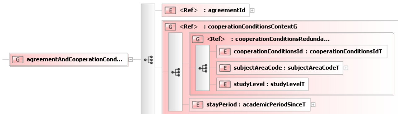
Figure 6.22: agreementAndCooperationConditionsContextG group
