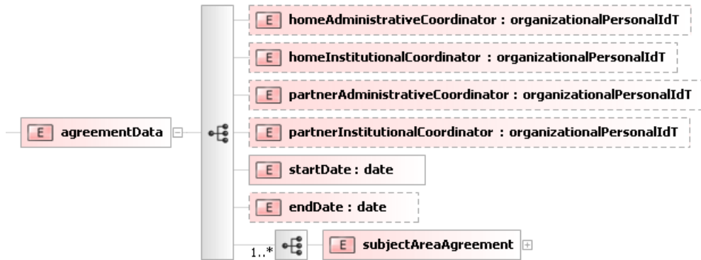
Figure 6.18: agreementData type
