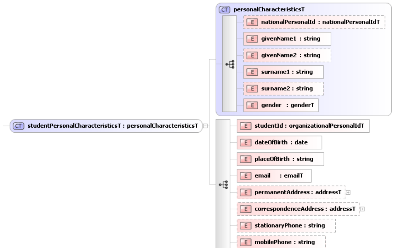
Figure 6.10: studentPersonalCharacteristicsT type
