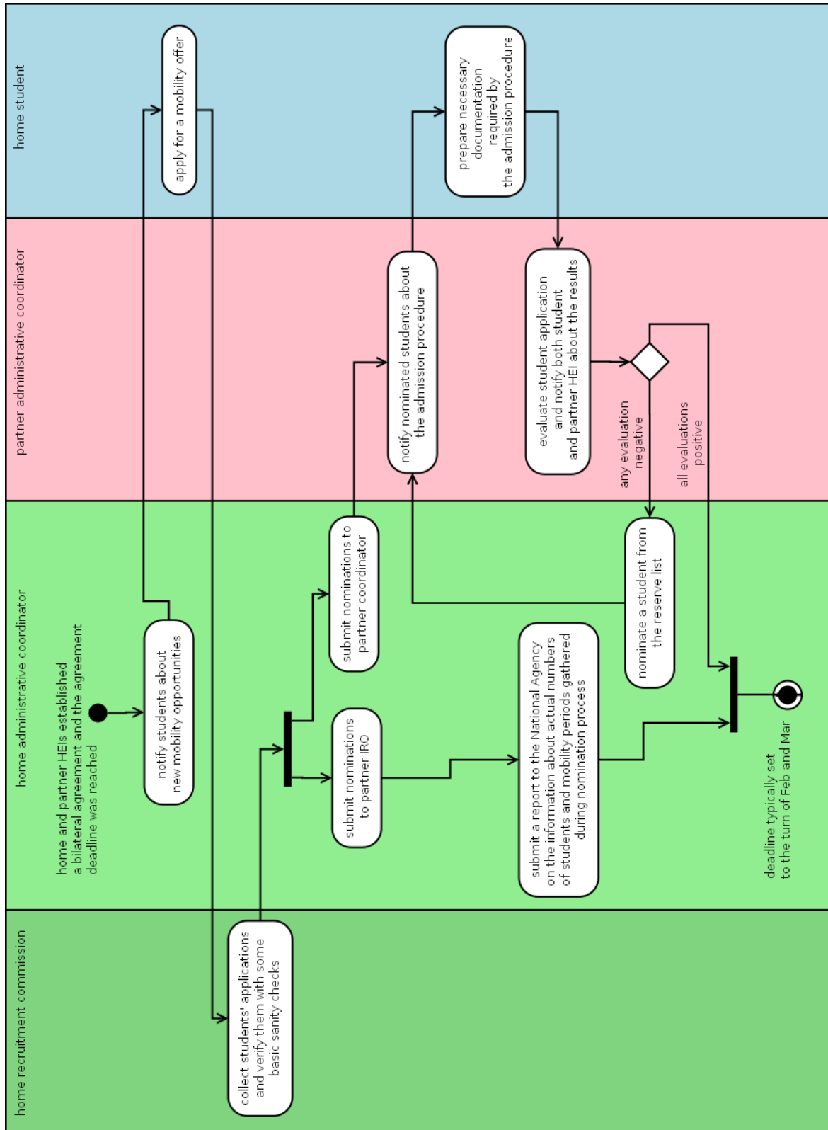
Figure 3.2: Making nominations
