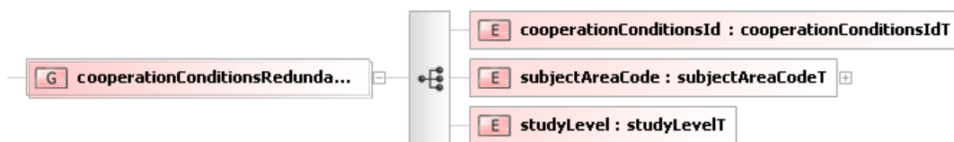
Figure 6.23: cooperationConditionsRedundantContextG group
