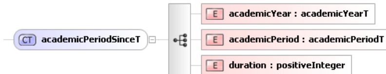
Figure 6.3: academicPeriodSinceT type
