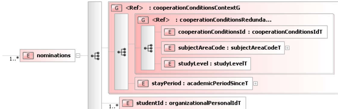
Figure 6.24: nominations element
