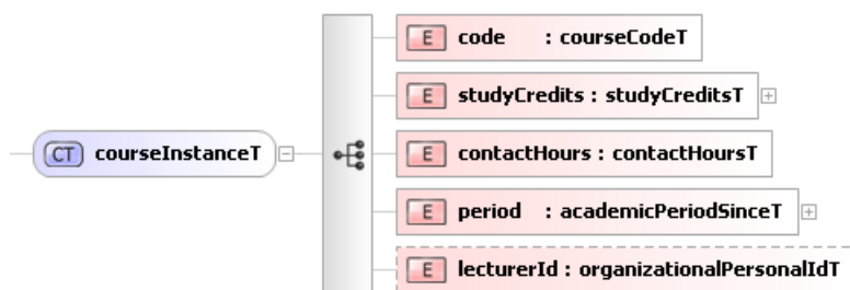
Figure 6.15: courseInstanceT type
